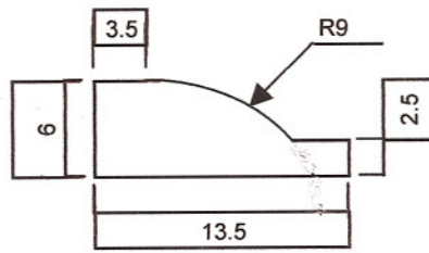
Profile of Type 1 loose sticking
