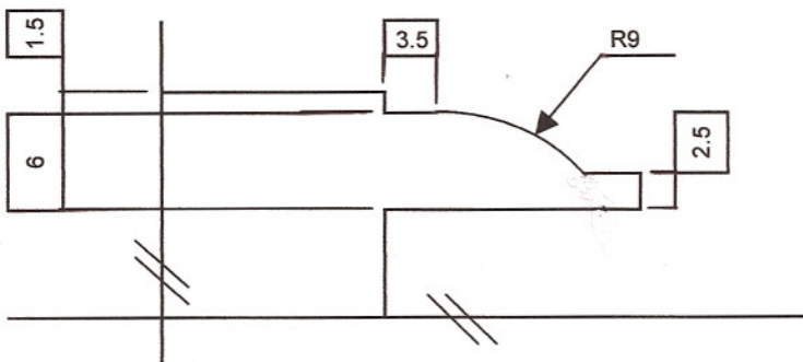
Profile of fixed sticking on stiles and rails
