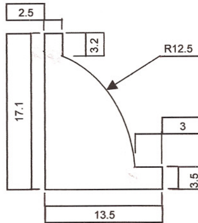
Profile of Type 2 loose sticking
