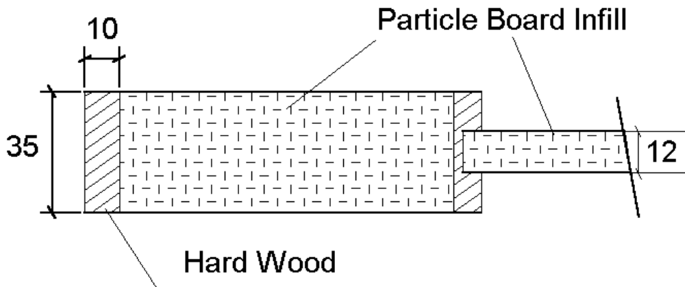
SECTIONAL PLAN
